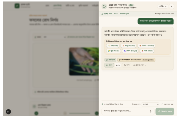
Figure 5: Text-image mismatch badge state (S3). Disagreement between user text and photograph raises an interactive warning badge, halting chemical recommendations until the farmer confirms the crop.
