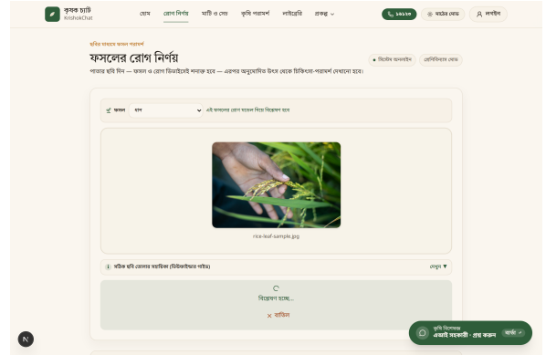
Figure 4: Photo-driven crop constraint state (S2). On-device visual inference predicts the crop species from a leaf photograph and scopes BM25 evidence retrieval strictly to the verified species manual.
